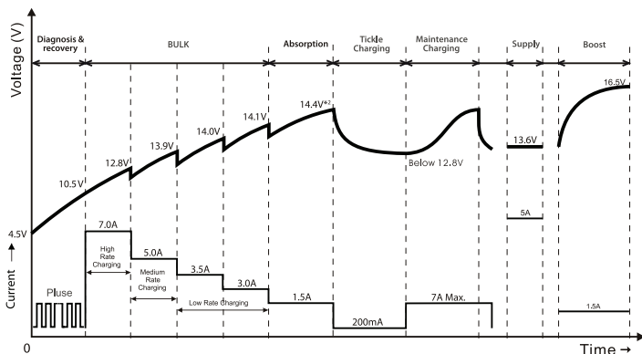
12V Battery Charging Curve
