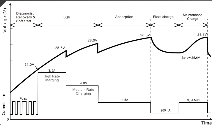
24V Battery Charging Curve
